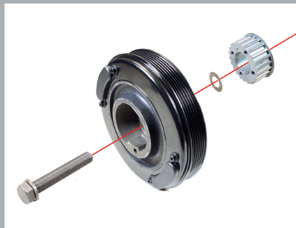
Image 1: crankshaft vibration damper with crankshaft central bolt and diamond washer
