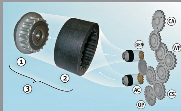
Figure 1: Over-running alternator pulley with flexible coupling sleeve and spur gear
