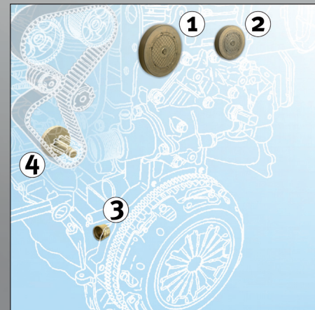
Fig. 2: Installation position
