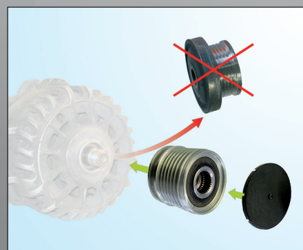
Fig. 3: Replacement procedure
