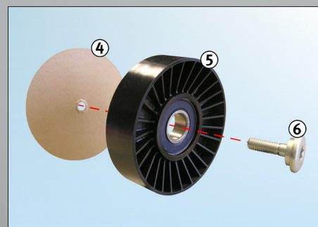
Figure 1: 55911 (new design)
