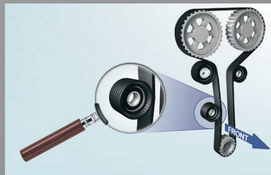
Figure 1: Belt path and pulley positions in the F4R engine
