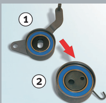
Image 1: Replaced tensioner pulley 55316 (1) and its successor 55383 (2)
