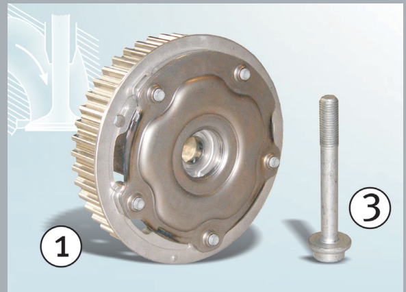
Image 1: Camshaft phasing unit for the intake side 205302 and central bolt 41301*
