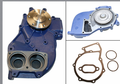
Figure 1: Water pump 65135 (without thermostats)
