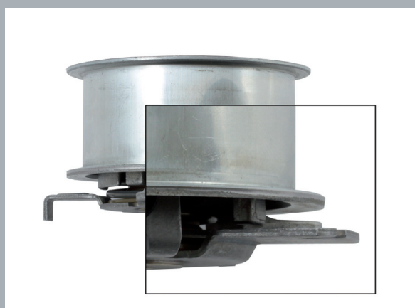
Image 2: Tensioner pulley in the installation position
