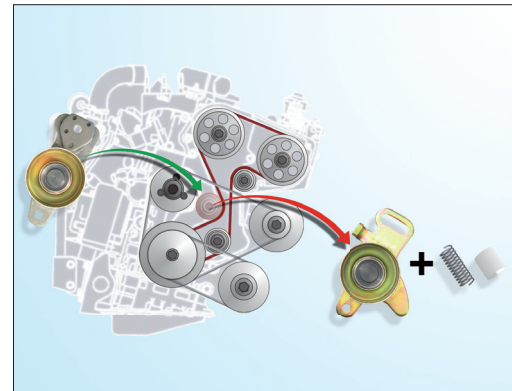
Pic. 2: Belt drive layout
