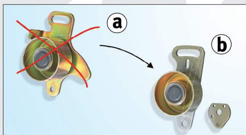
Pic. 1: Replaced and new tension roller design
