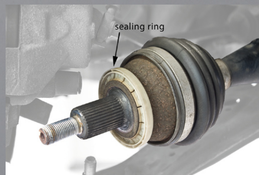
Figure 1: The sealing rings could differ in design and colour!
